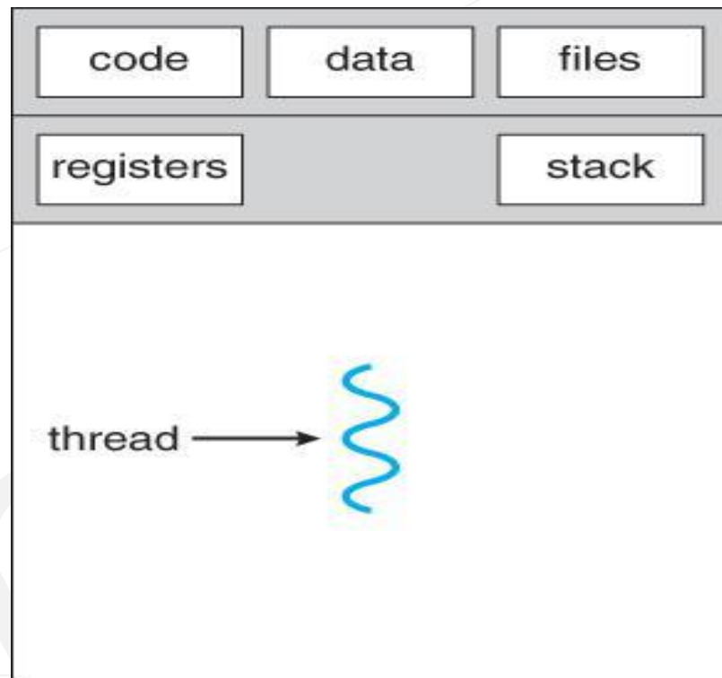
single-threaded process
