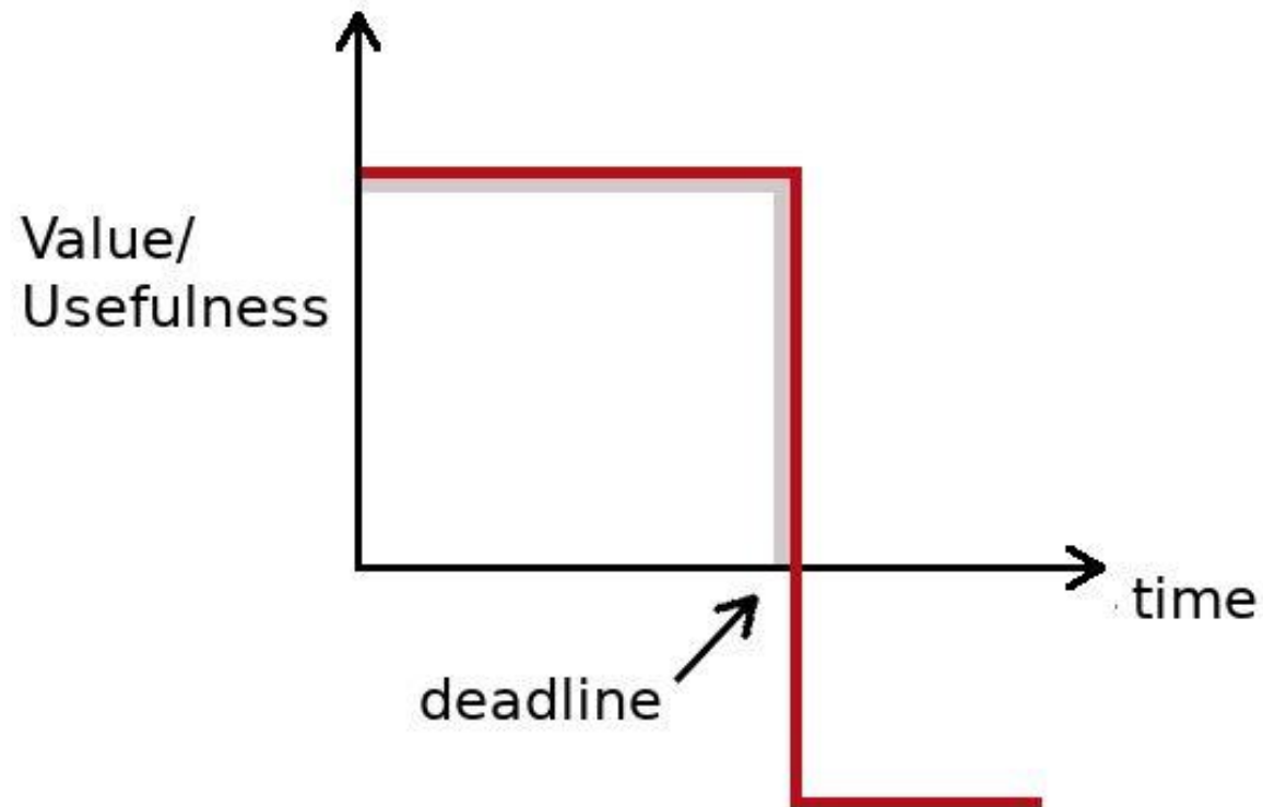
hard real-time
