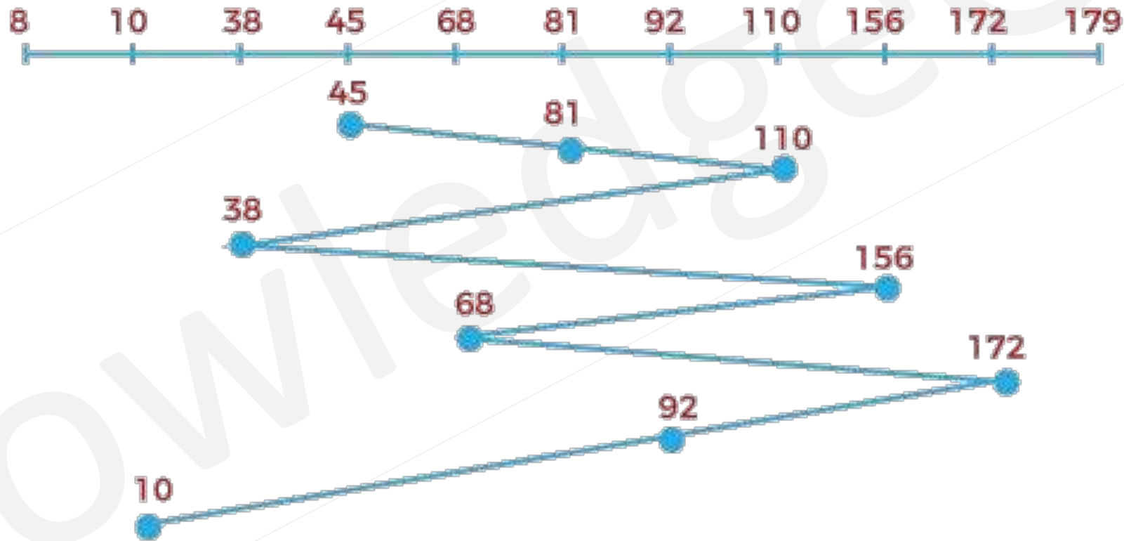
FCFS Disk Scheduling Algorithm
