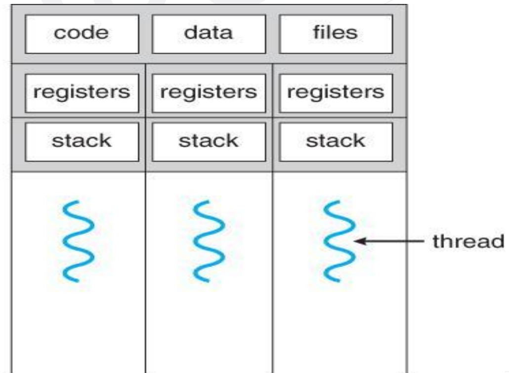
multithreaded process
