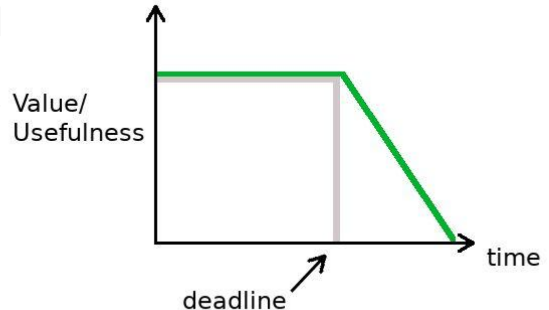
soft real-time
