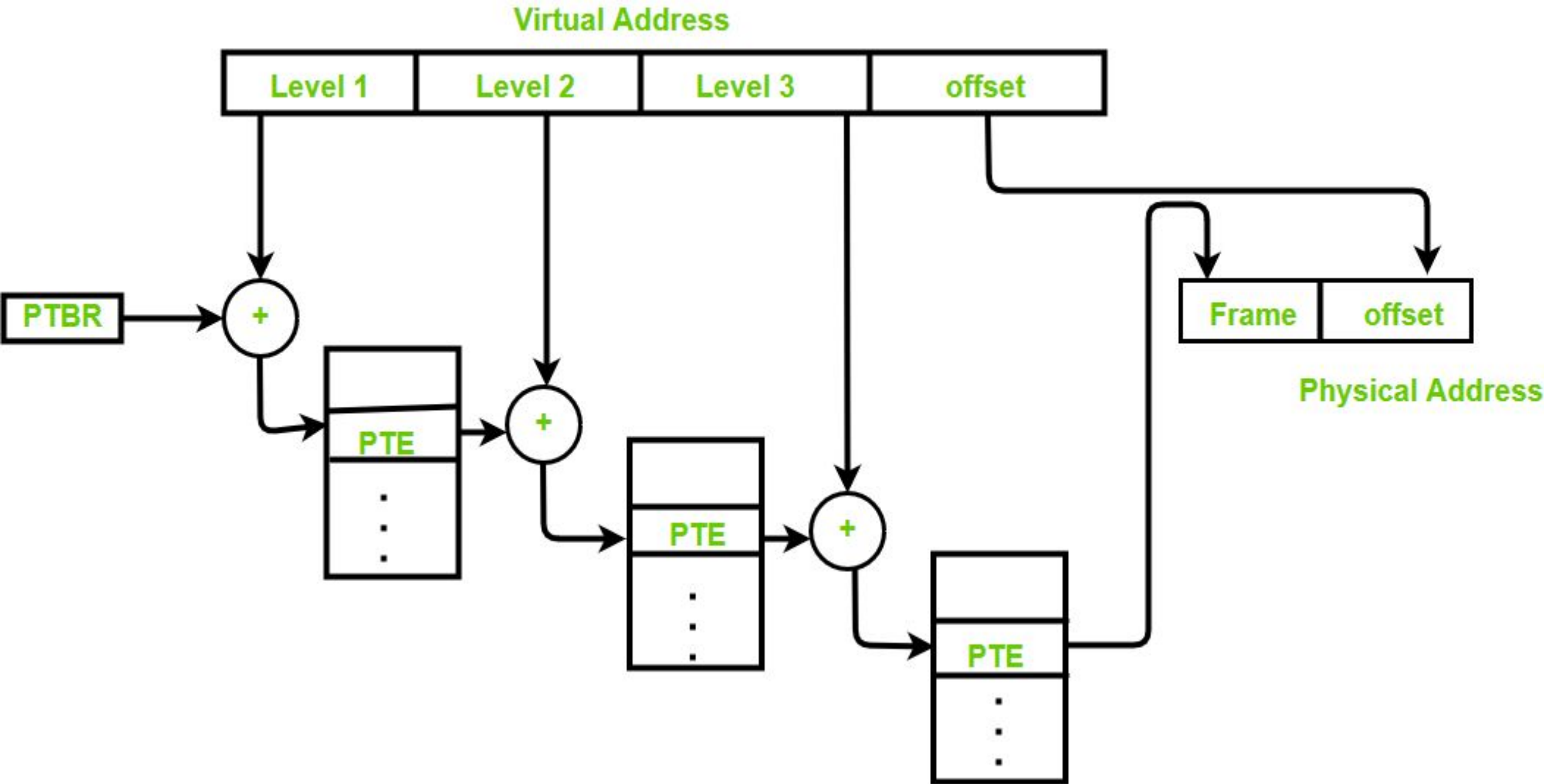
3 Level paging system
