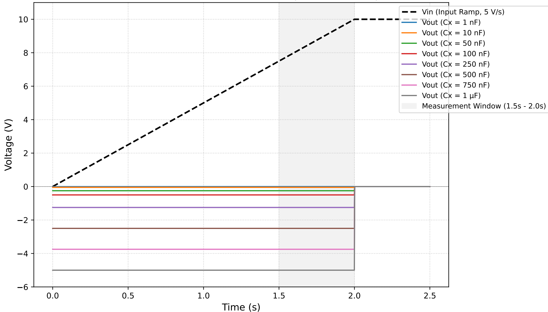
C/V Converter Simulation: Vin Ramp & Vout Sweep
