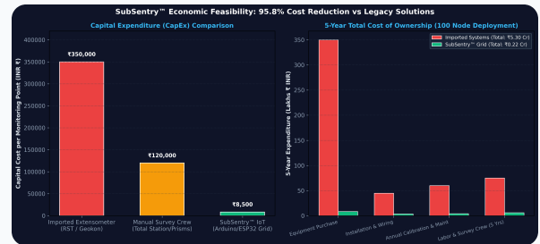
Fig 5.1: 5-Year Colliery Total Cost of Ownership (TCO) Comparison
