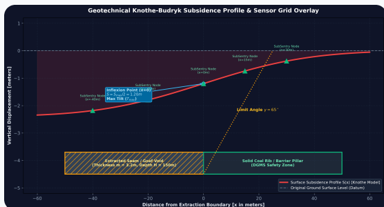
Fig 4.1: Knothe-Budryk Surface Trough Curve S(x) Over Extraction Goaf
