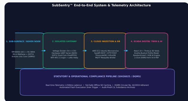
Fig 1.1: End-to-End Edge-to-Cloud Telemetry Pipeline Architecture
