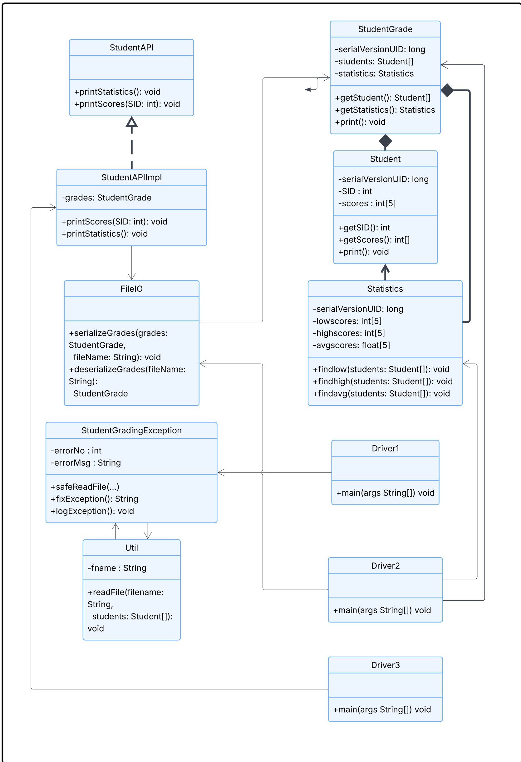
Class Diagram – Adapter, Driver, Model, Util, Exception
