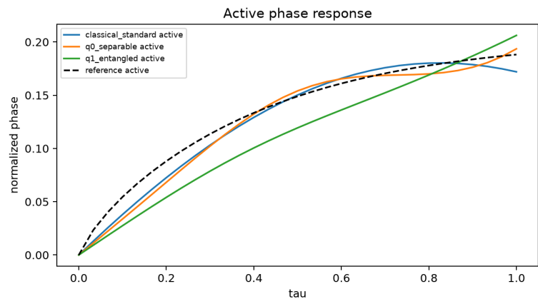
Figure 11. Active-waveguide normalized phase response.
