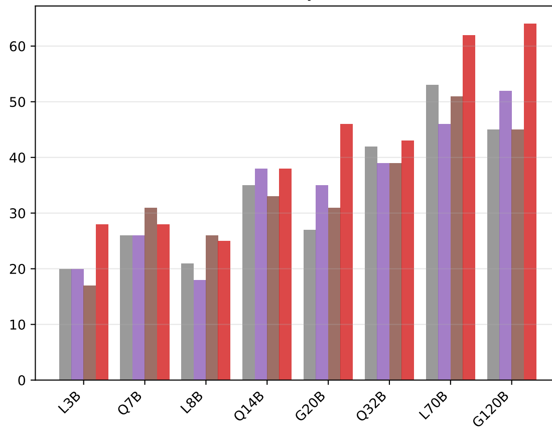
GPQA
