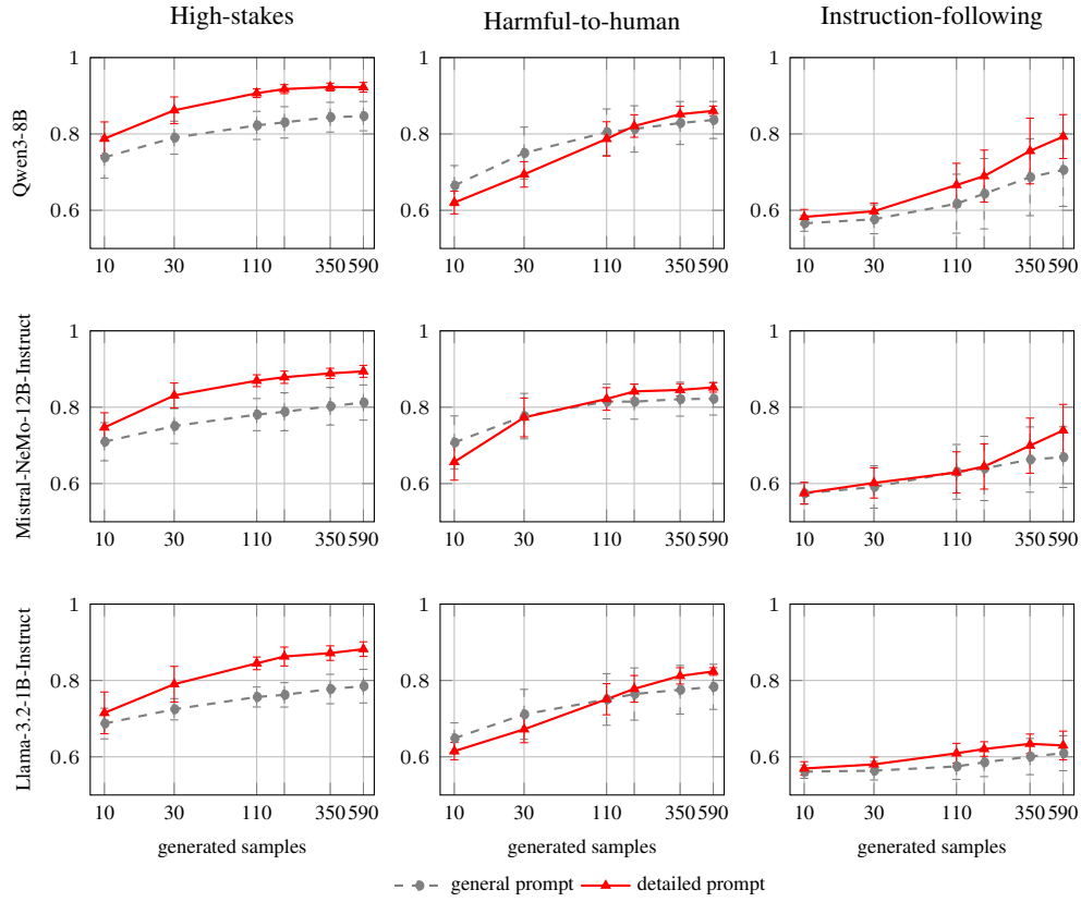
Figure 7: Direct-prompting learning curves on three further probe models (rows) for the three concepts (columns): mean AUROC over the concept’s evaluation splits vs. generated samples, averaged over the four generators, under the general (grey, dashed) and detailed (red) prompt. Error bars are the standard deviation over draws and generators.
