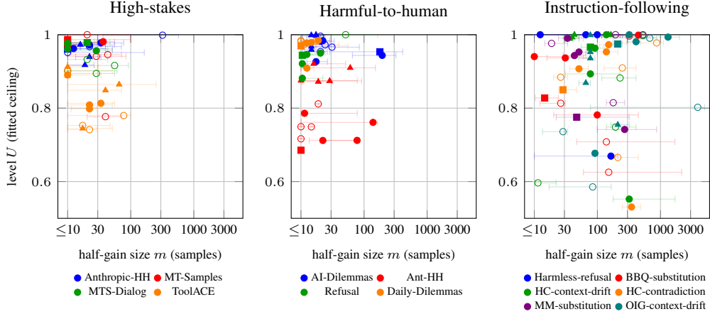
Figure 2: Level against half-gain size. Every Gemma-3-27B-IT learning curve as one point: fitted level U vs. half-gain size m (log scale; m below the smallest measured size is drawn at 10), coloured by evaluation split; \circ general prompt, \bullet detailed prompt, \blacktriangle LLM-written prompt, \blacksquare split-targeted set; bars are 95% bootstrap intervals of m where they span less than a factor of 100. Values in Table 7.
