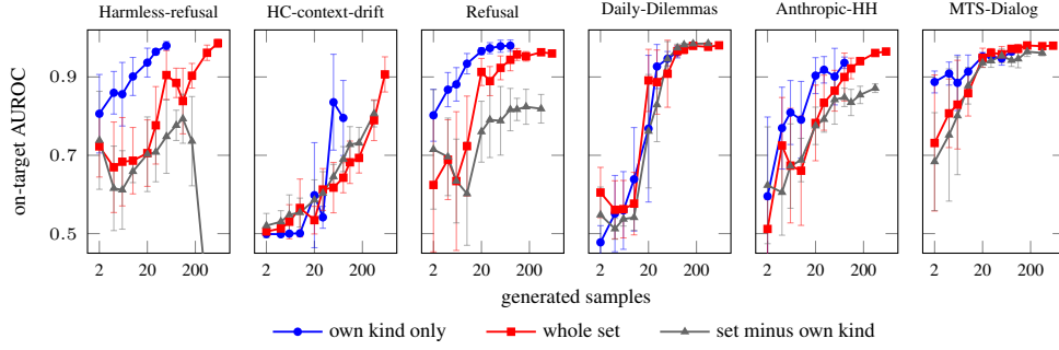
Figure 3: Coverage test. Kind-only, whole-set, and set-minus-kind curves on the target split, cut from DeepSeek-V4-Pro’s detailed set, eight draws per size (bars: standard deviation). Left two panels: instruction splits, which reach their level from tens of samples of their own kind and slowly or not at all from the rest of the set; middle two: harmful and right two: high-stakes splits, which reach it either way. Every split is in Table 11.
