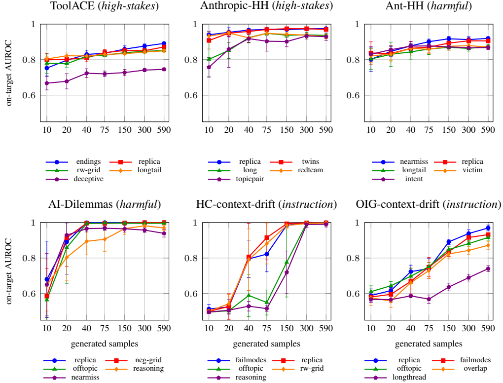
Figure 8: Five LLM-written prompts per split. On-target AUROC of a probe fit on n samples of one prompt’s set and nothing else, one line per prompt, for six evaluation splits across the three concepts; eight class-balanced draws per size, error bars are the across-draw standard deviation, sizes below 49 use a single accumulation step. Table 16 in Appendix K expands the legend abbreviations and lists the values and per-prompt saturation points.
