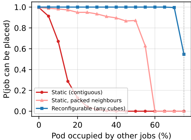
(a) Can a 1024-chip job start?
