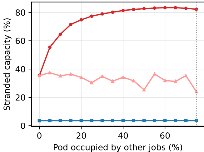
(b) Free capacity left after the largest job
