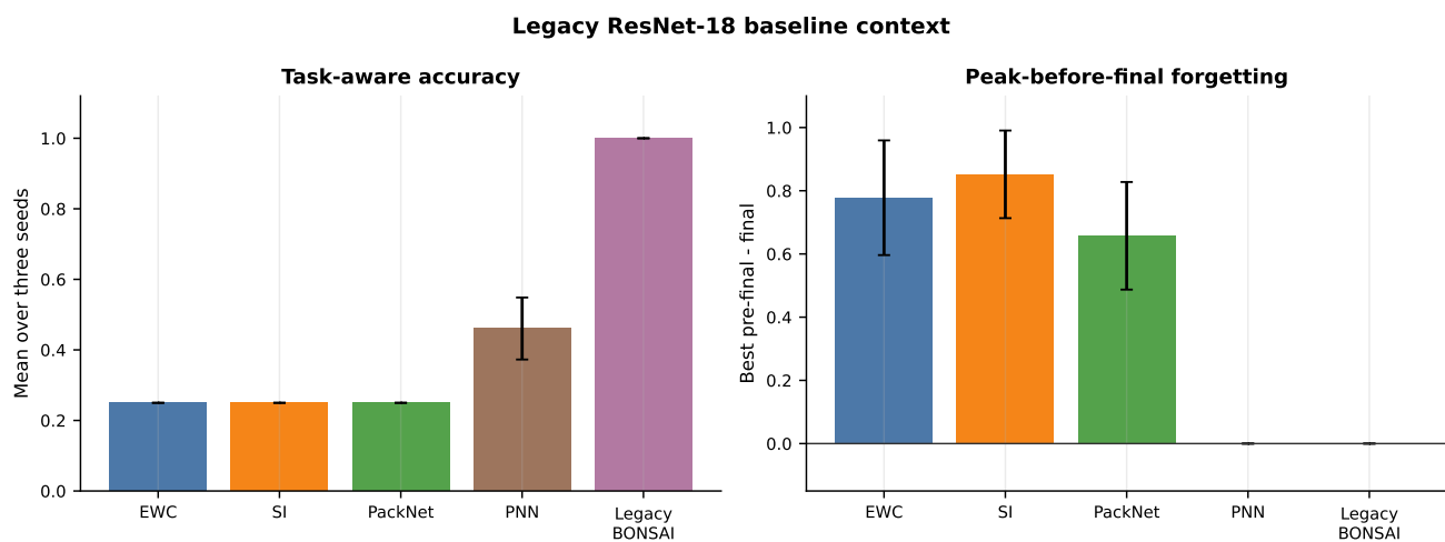
Fig. 9. Corrected legacy ResNet-18 context comparison. The established baselines and legacy BONSAI are intentionally separated from the capacity-mismatched new modular results.
