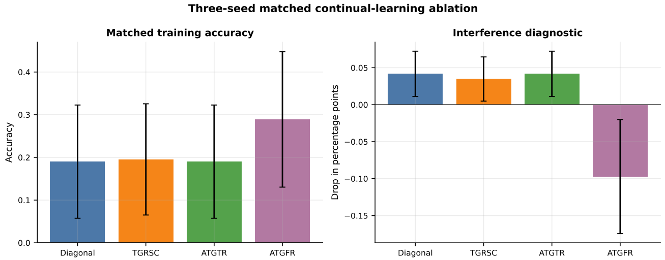
Fig. 7. Matched consolidation ablation against the modular controls. The factorial component study is shown separately in Fig. ??.
