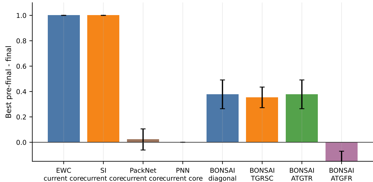
Peak-before-final forgetting
