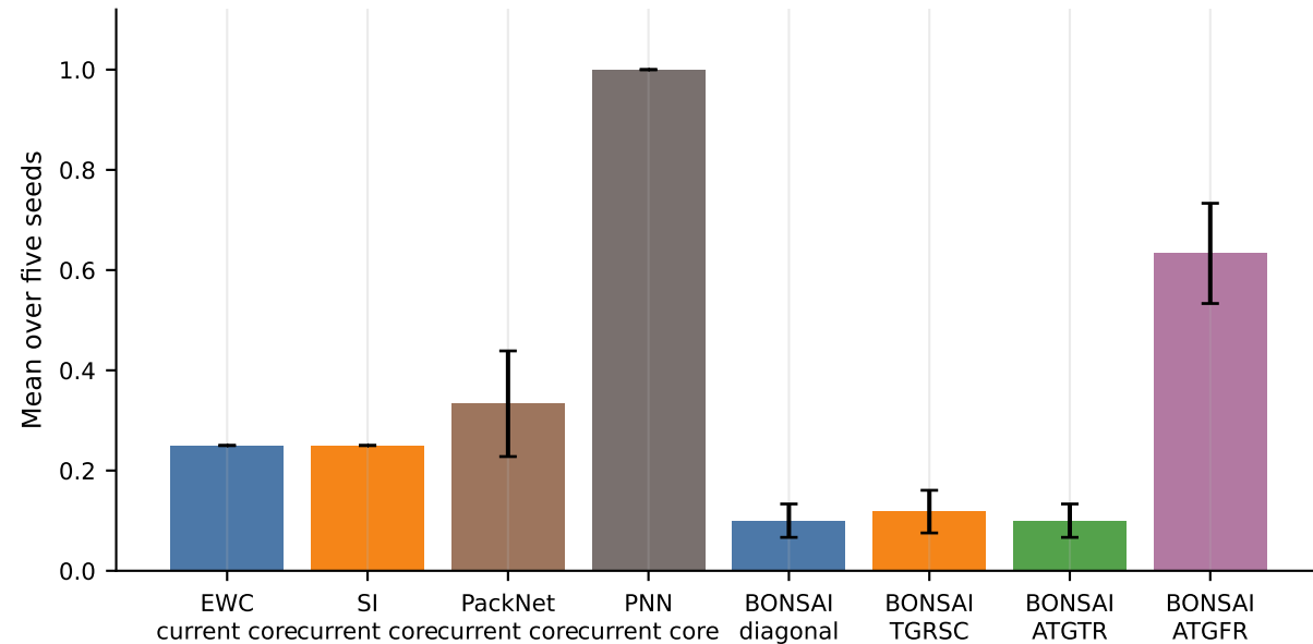
Task-aware accuracy
