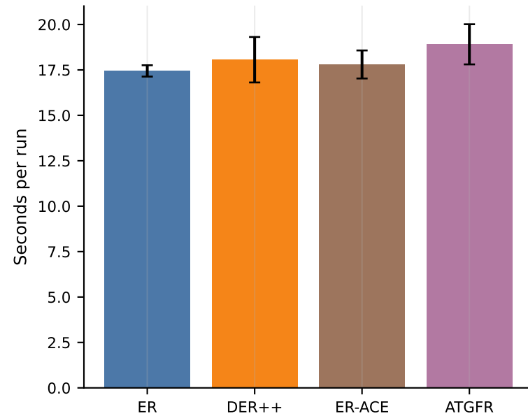
Wall-clock cost
