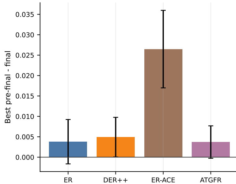
CIFAR-100 forgetting
