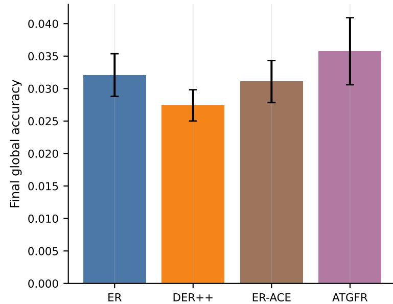
CIFAR-100 accuracy
