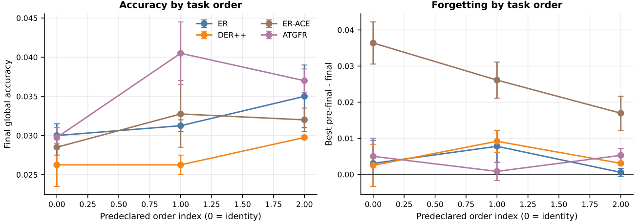
Fig. 4. All three predeclared task orders in the Split-CIFAR-100 study. Error bars are standard deviations over the two seeds.
