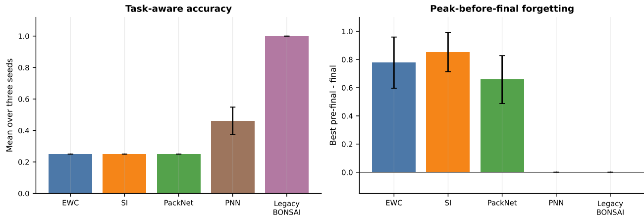
Fig. 9. Corrected legacy ResNet-18 context comparison. The established baselines and legacy BONSAI are intentionally separated from the capacity-mismatched new modular results.
