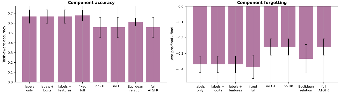
Fig. 8. Factorial ATGFR component ablation. The result supports replay but does not justify claiming that every exotic descriptor improves accuracy.
