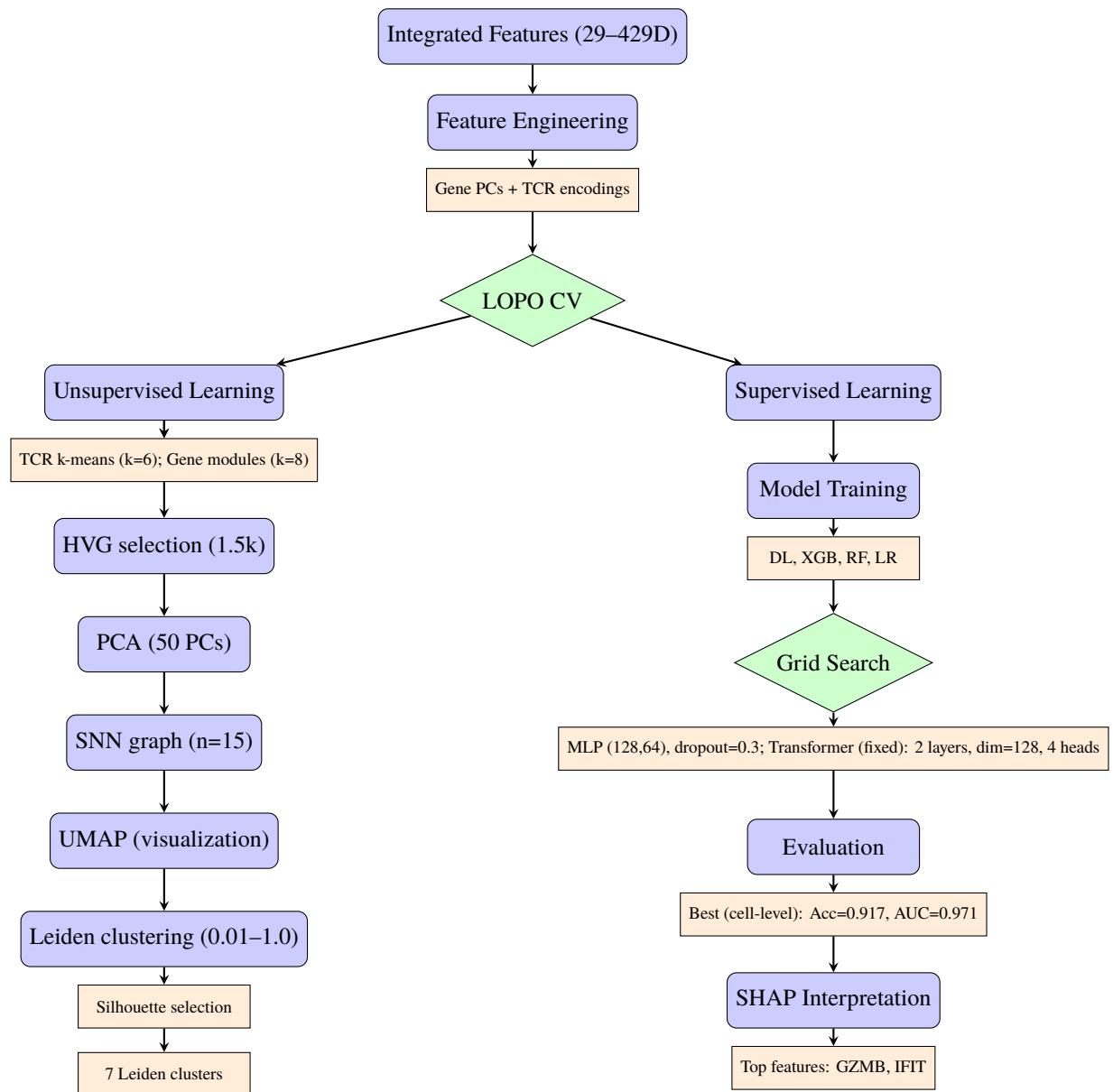
Figure 1: Enhanced Modeling Pipeline: Two-stage strategy with feature engineering, hyperparameter optimization via grid/randomized search, and LOPO cross-validation. Representative deep model hyperparameters (MLP selected via inner CV; CNN/BiLSTM/Transformer used fixed representative configurations) and Leiden clustering outputs (target: 7 clusters, silhouette-optimized resolution) are shown.
