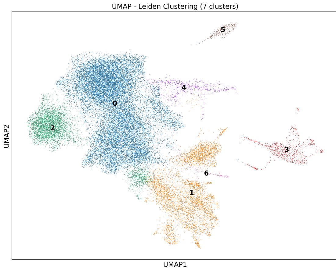
(b) UMAP visualization of Leiden clusters colored by cluster assignment.
