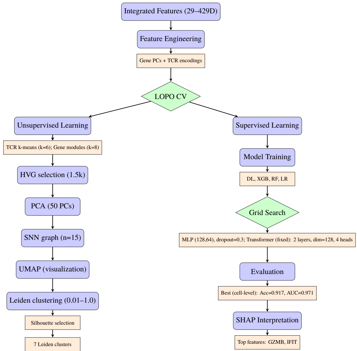
Figure 2: Enhanced Modeling Pipeline: Two-stage strategy with feature engineering, hyperparameter optimization via grid/randomized search, and LOPO cross-validation. Representative deep model hyperparameters (MLP selected via inner CV; CNN/BiLSTM/Transformer used fixed representative configurations) and Leiden clustering outputs (target: 7 clusters, silhouette-optimized resolution) are shown.
