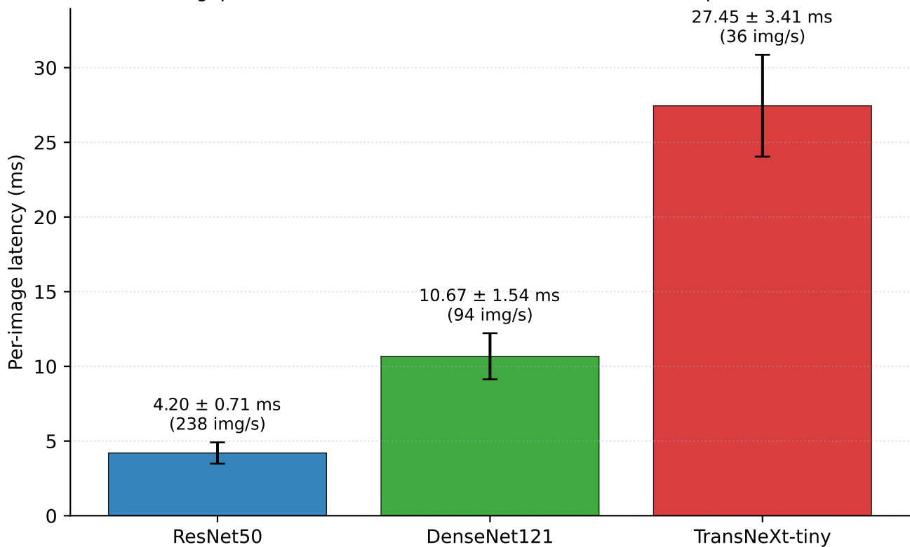
Inference throughput on RTX 5070 (bf16-mixed, batch=1, 100 warmup / 1000 measurement)
