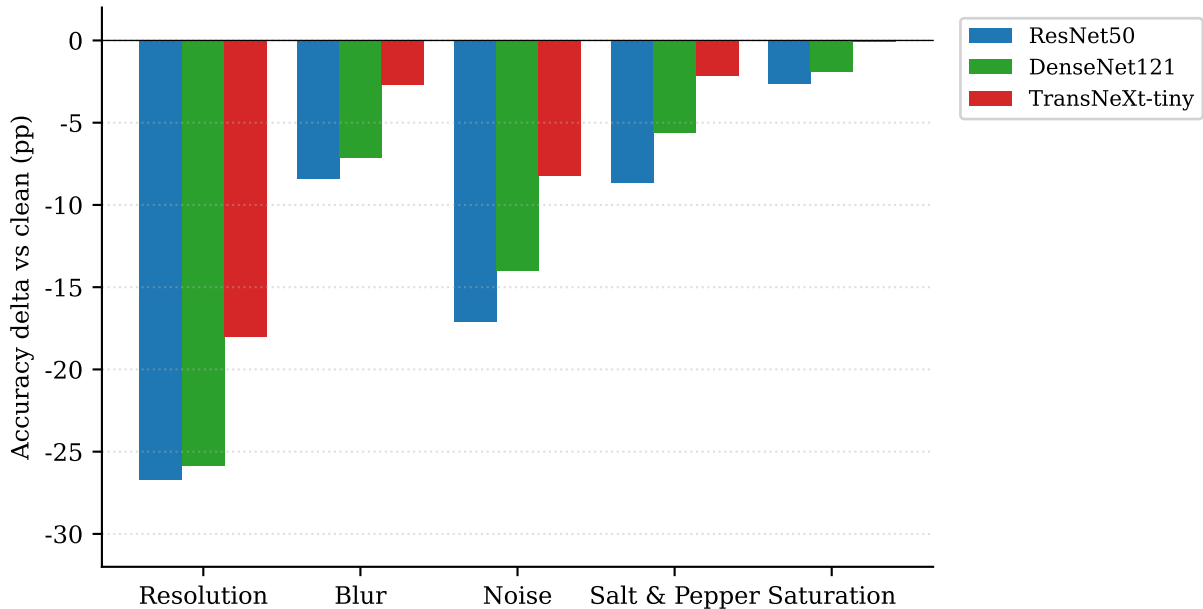
CIFAR-10 - per-axis attribution at L3
