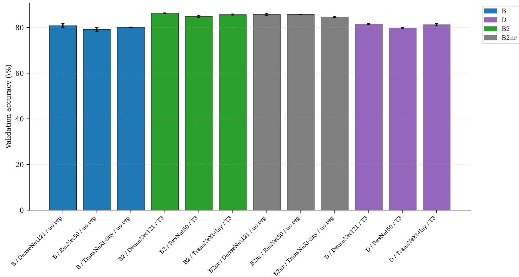
MNIST - multi-seed variance at L3 (mean \pm \sigma , n=3)
