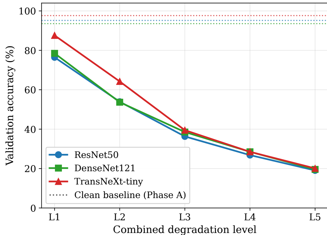
CIFAR-10
