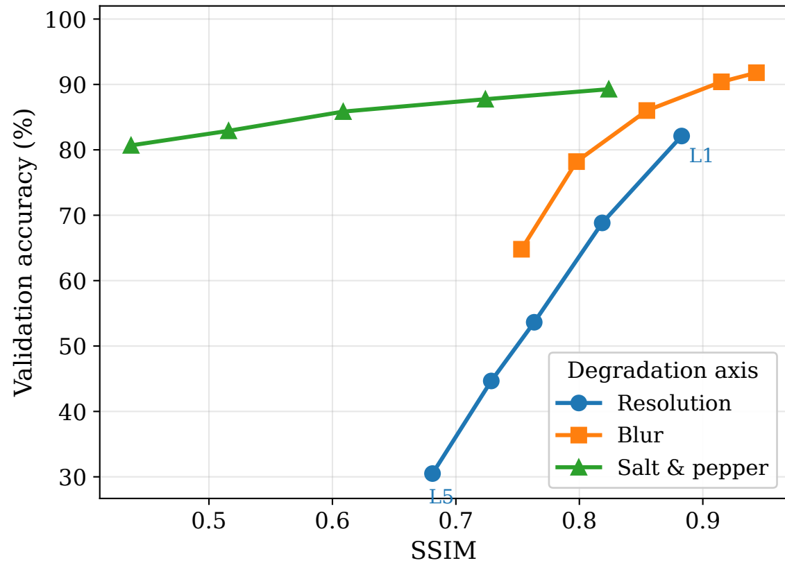
CIFAR-10
