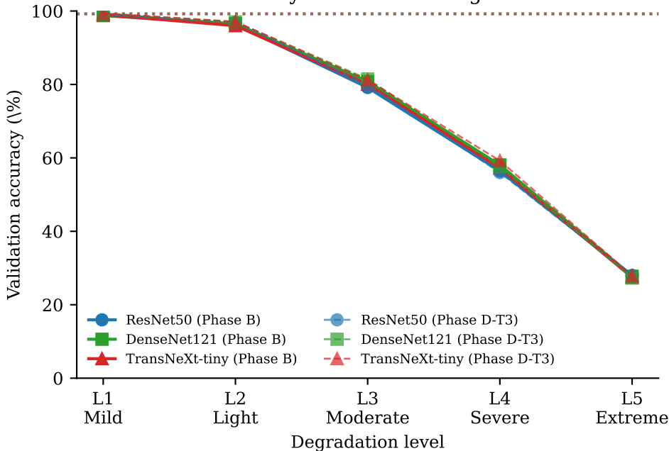
MNIST - accuracy vs combined degradation level
