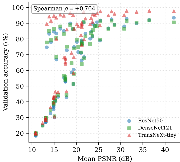
CIFAR-10
