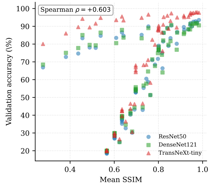
CIFAR-10
