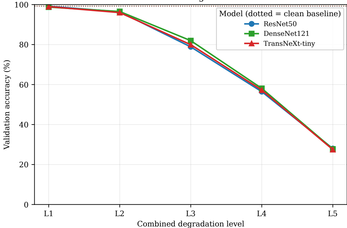
Phase B1 combined degradation -- MNIST
