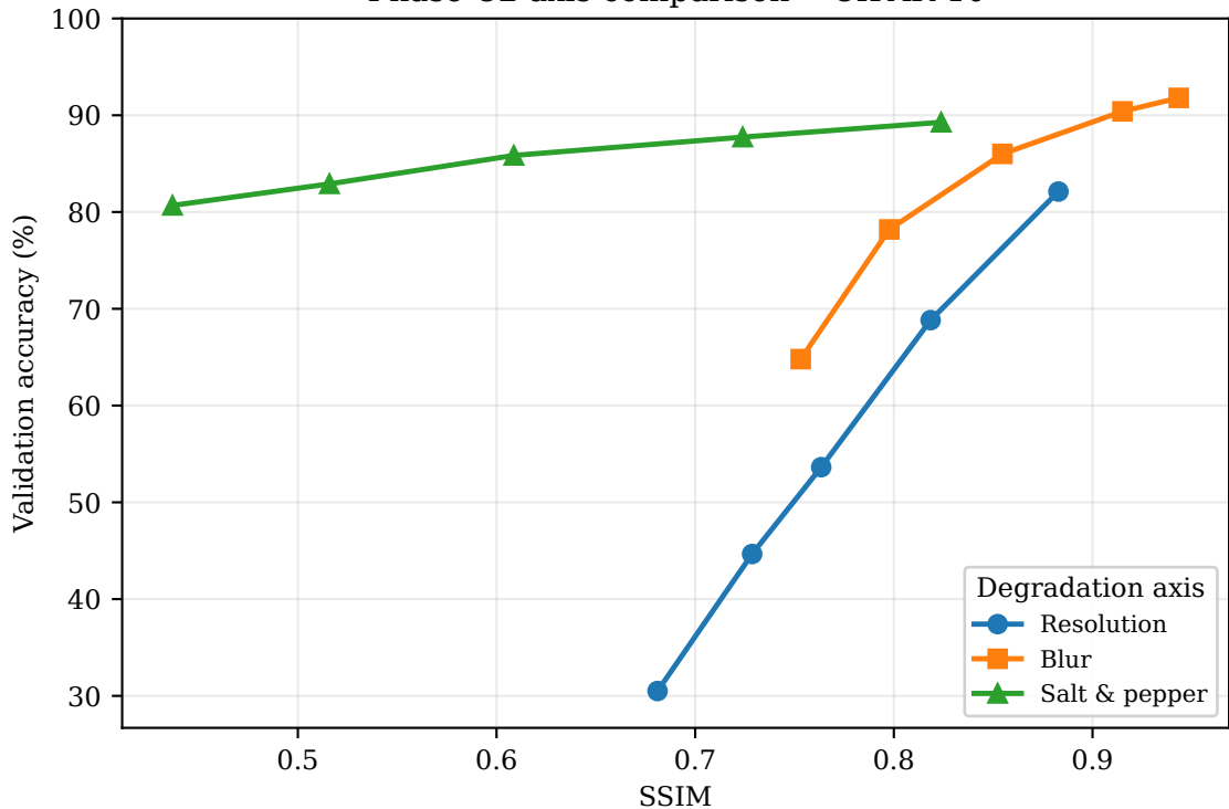
Phase C2 axis comparison -- CIFAR-10
