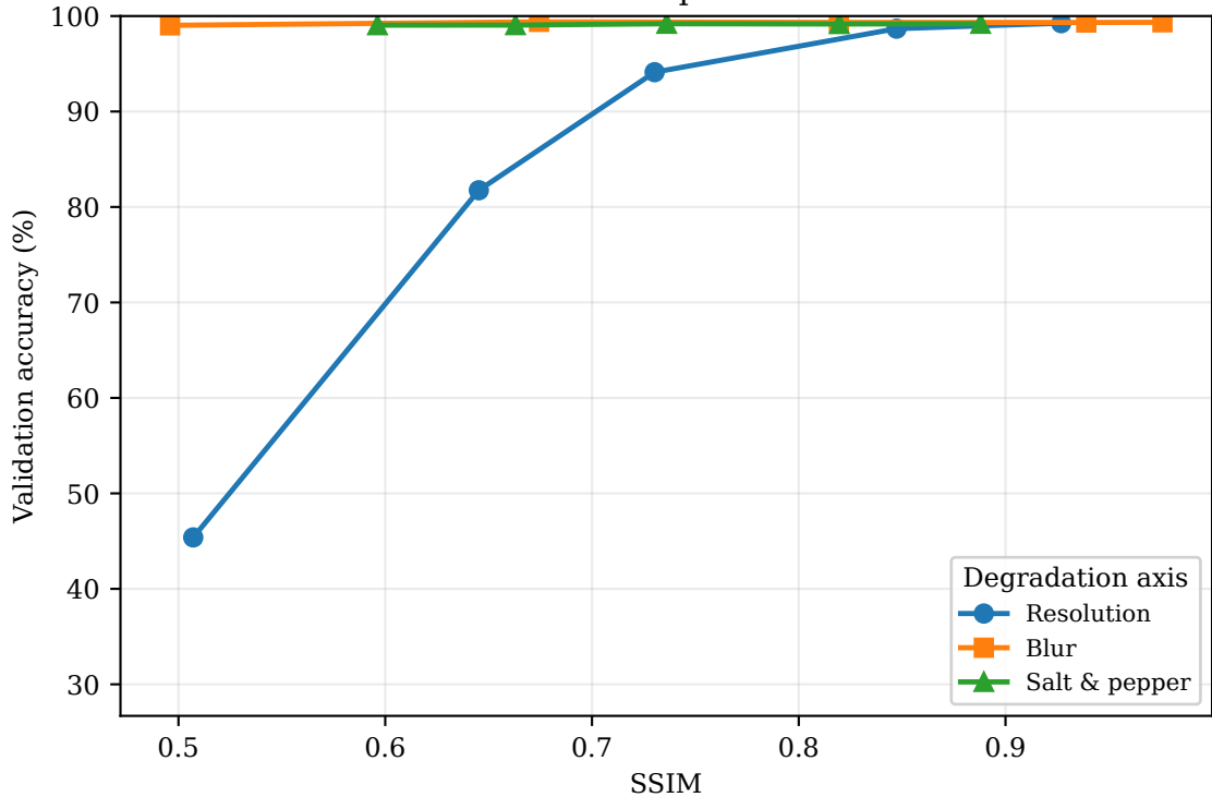
Phase C2 axis comparison -- MNIST
