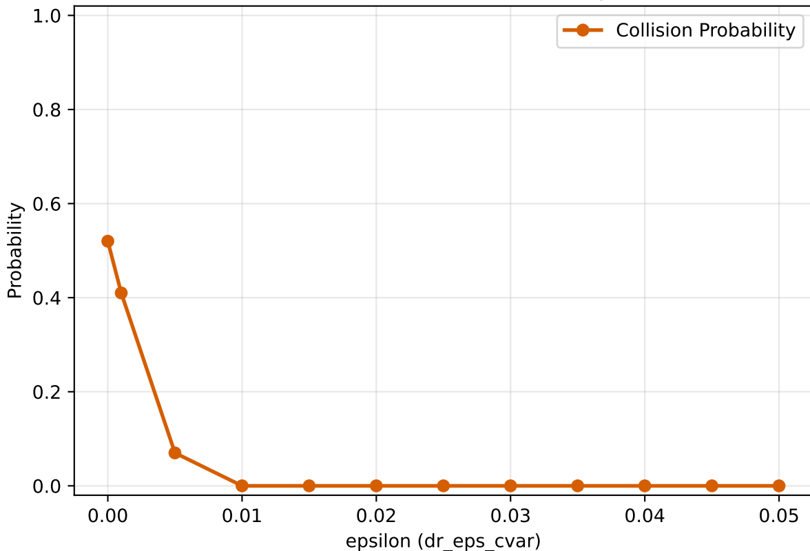
DR-MPPI Collision Probability vs Epsilon | Scenario 2
