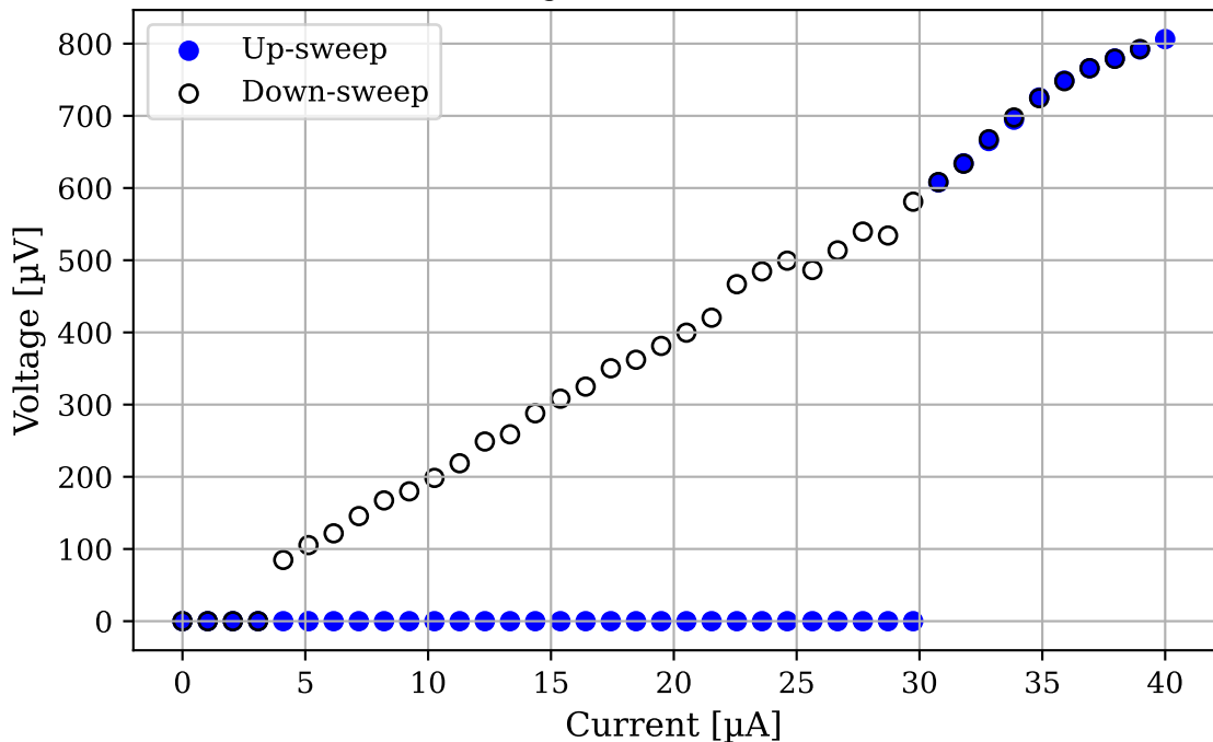
RCSJ model IV curve
