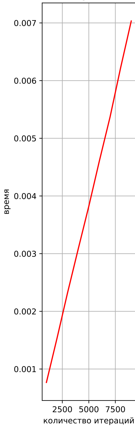
Integration
