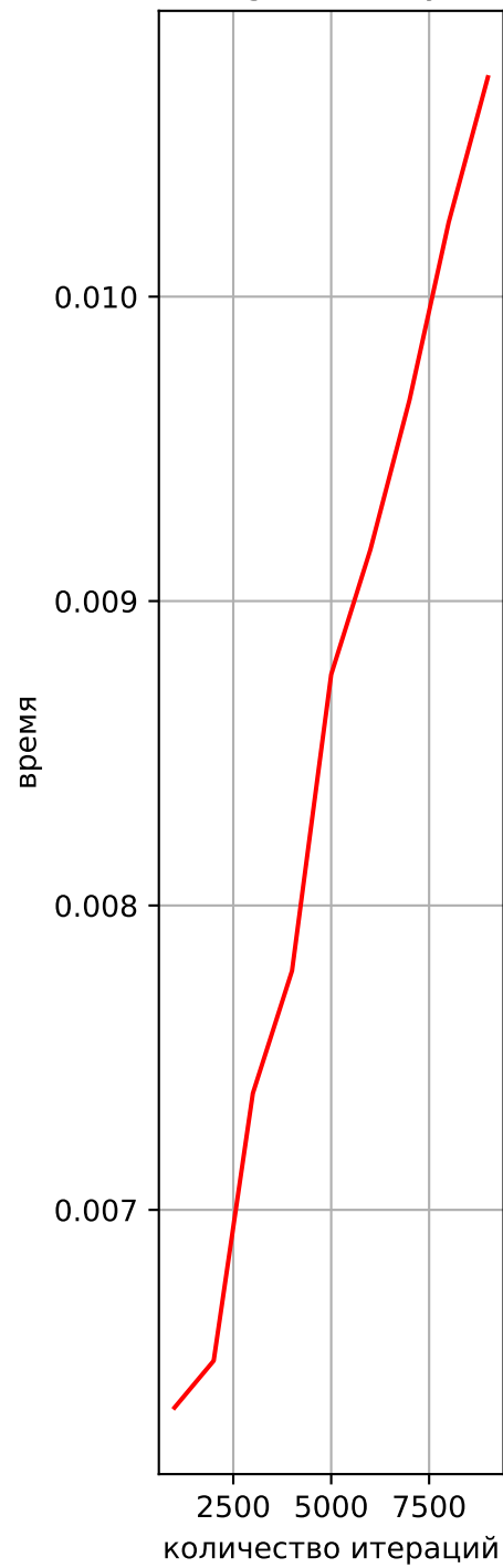
Integration Async
