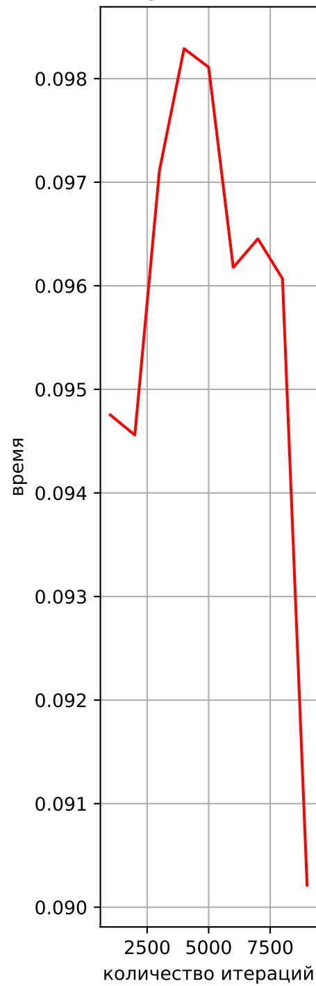
Integration Process
