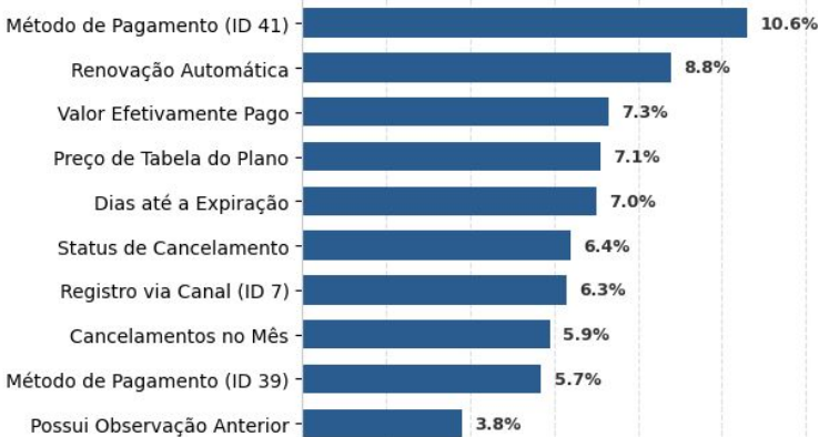
Feature Importance
