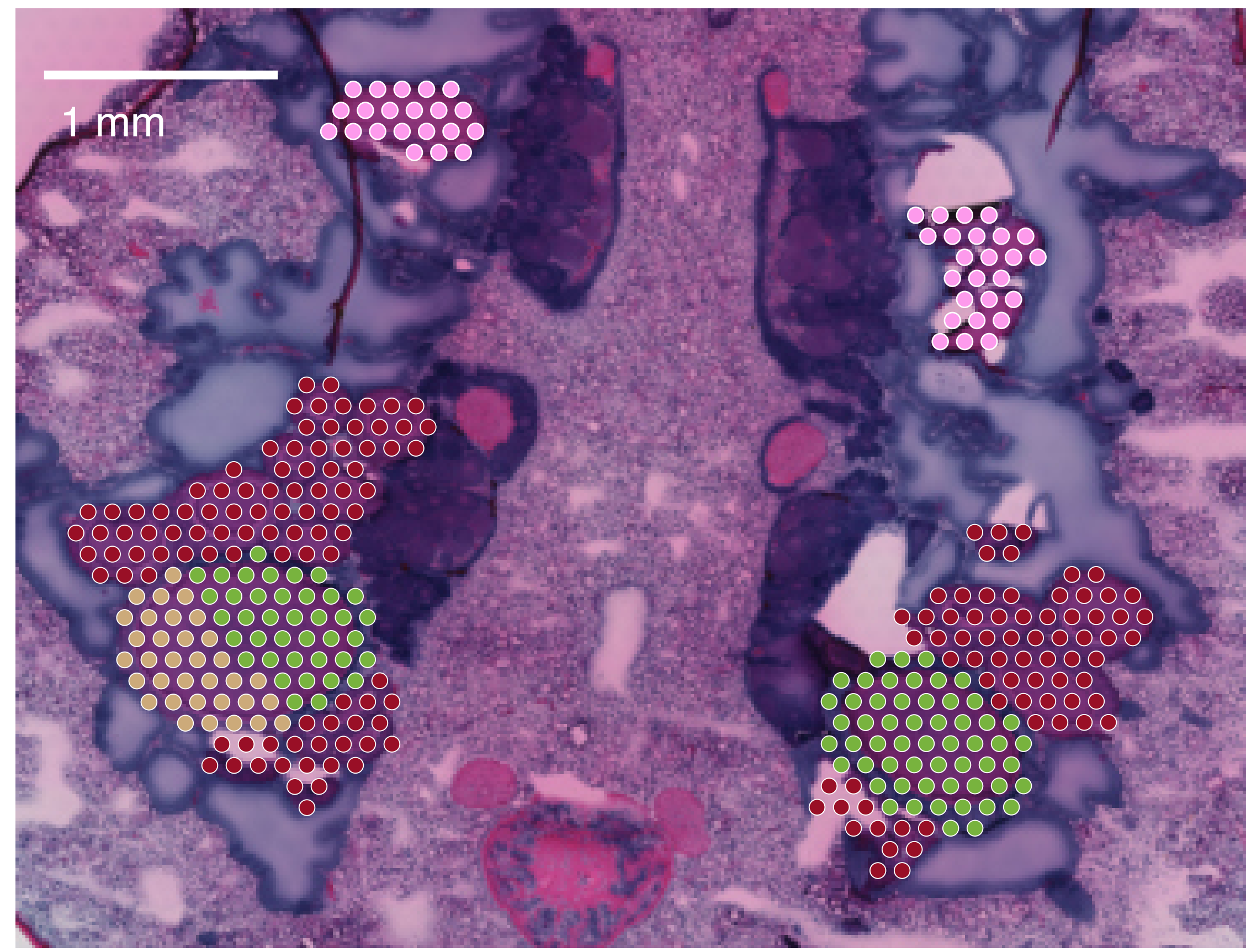
Manual curation
