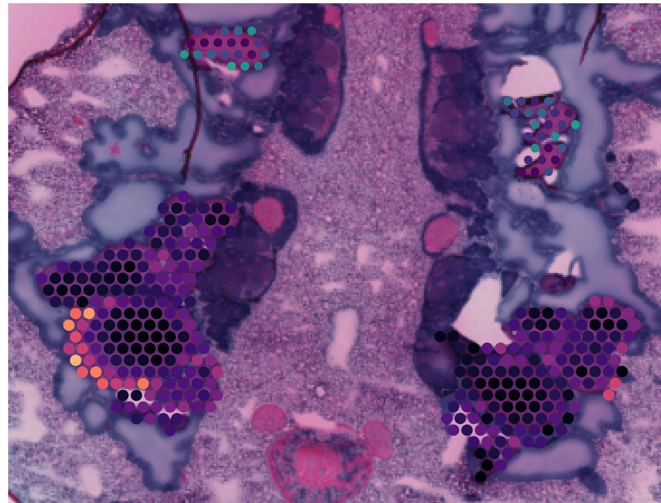
Manual curation
