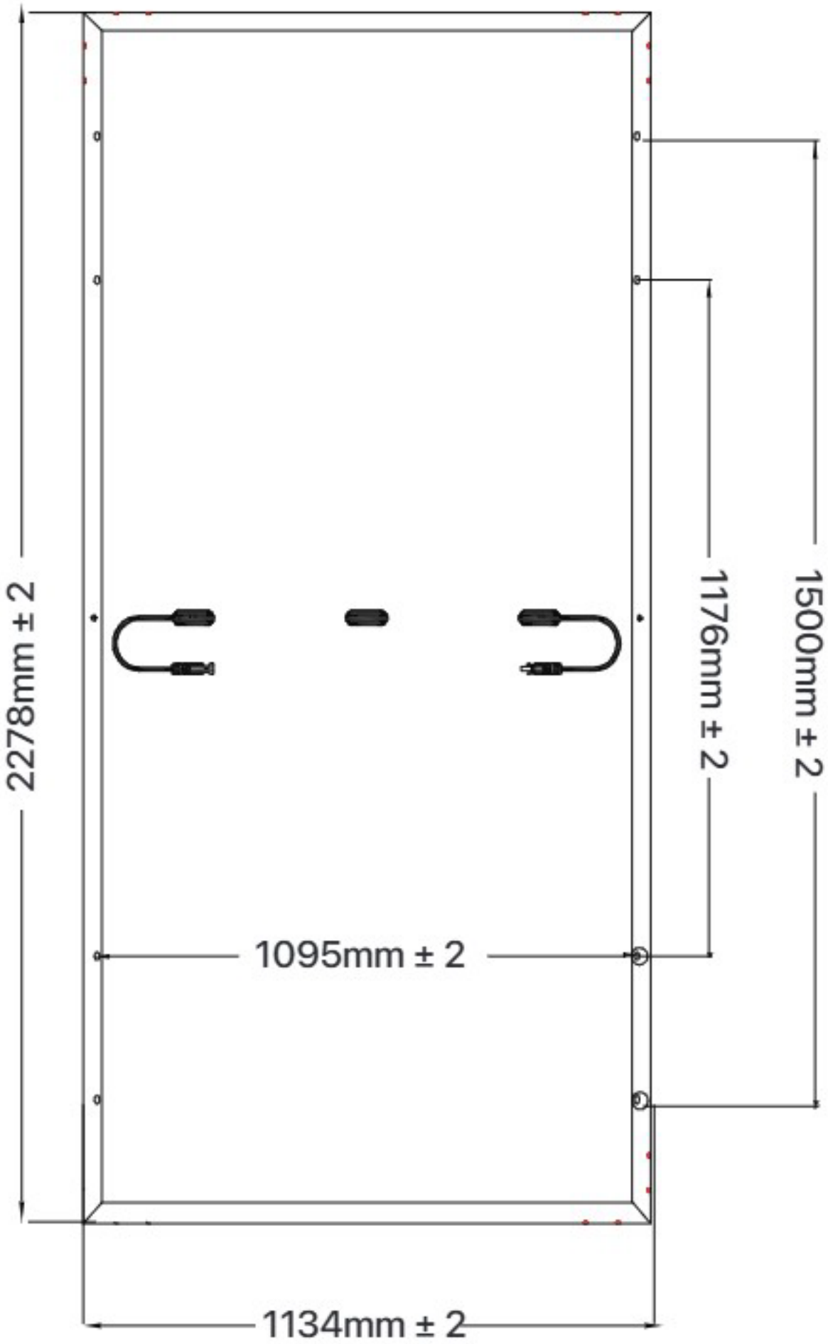
Mechanical Drawing
