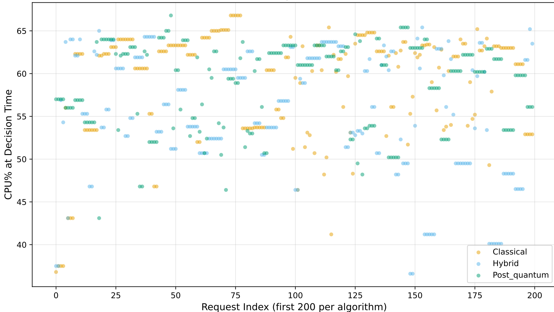
CPU Load vs Algorithm (55 users)
