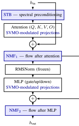
Fig. 1. One S^3 -adapted transformer layer. Frozen model components in black; learned S^3 adapters in blue (STB preconditioning, SVMO-modulated projections, NMF continuous flows). Residual connections shown at right.
