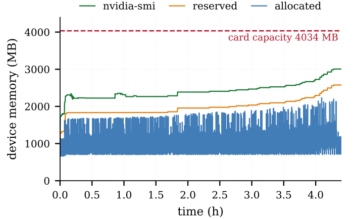
Fig. 2. Device memory over the full 4 h 16 min run of Qwen2.5-7B (114 766 samples at 100ms). The sawtooth is Algorithm 1 itself: each tooth is one LOAD–compute–FREE cycle of a 0.43 GB decoder layer. The model is 15.2 GB on disk, yet nothing approaches the card’s 4034 MB—the picture Theorem 7 predicts. The upward drift of the reserved curve is the caching allocator retaining freed blocks, not growth in what USF keeps resident.
