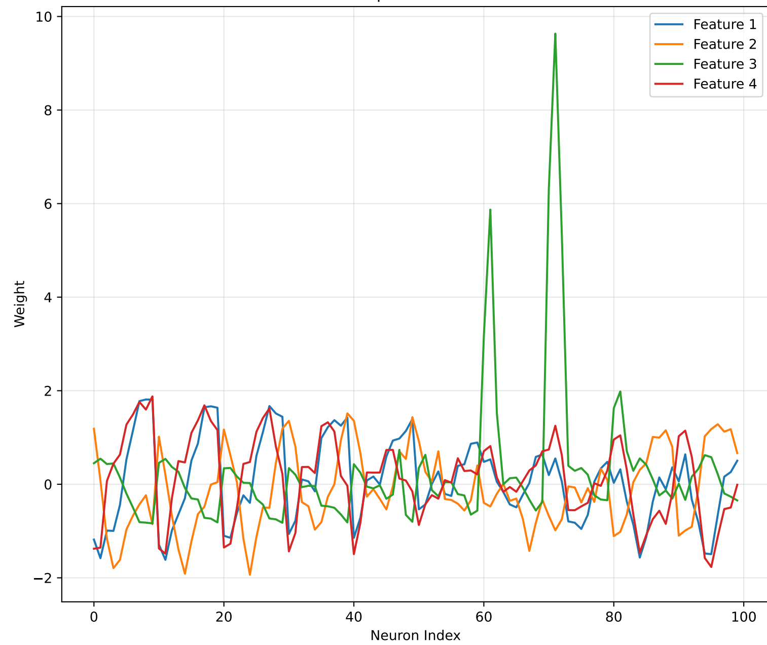
Component Planes
