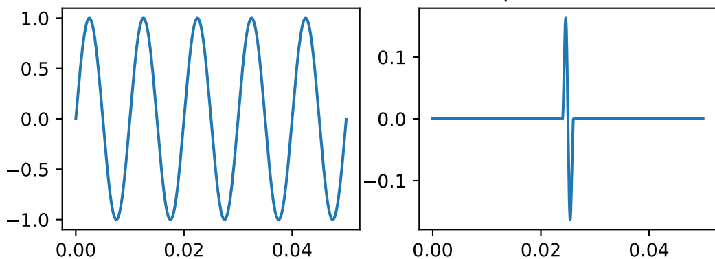
Semnal initial Semnal filtrat printr-o fereastra Hanning
