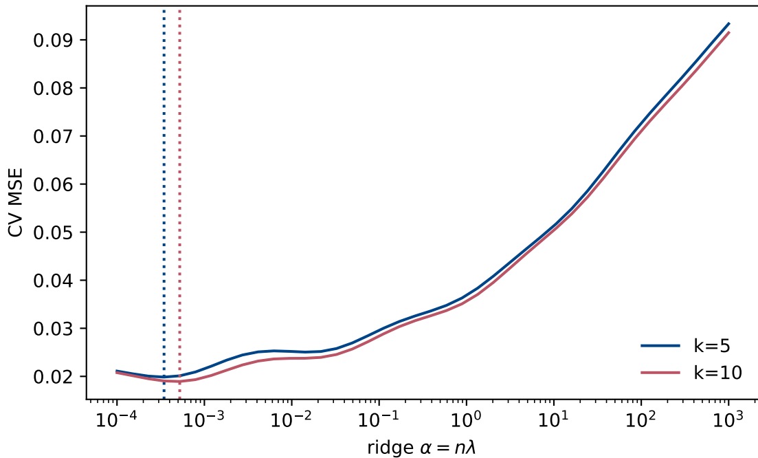
Ridge, degree 12
