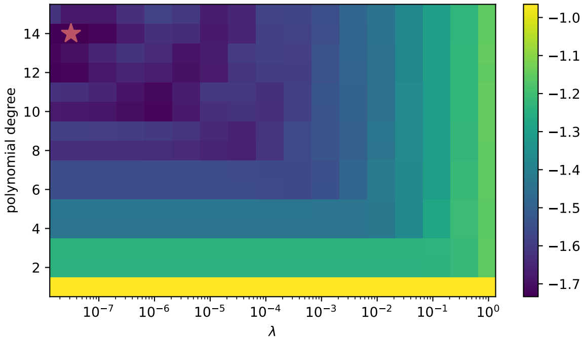
Ridge: log10 CV MSE
