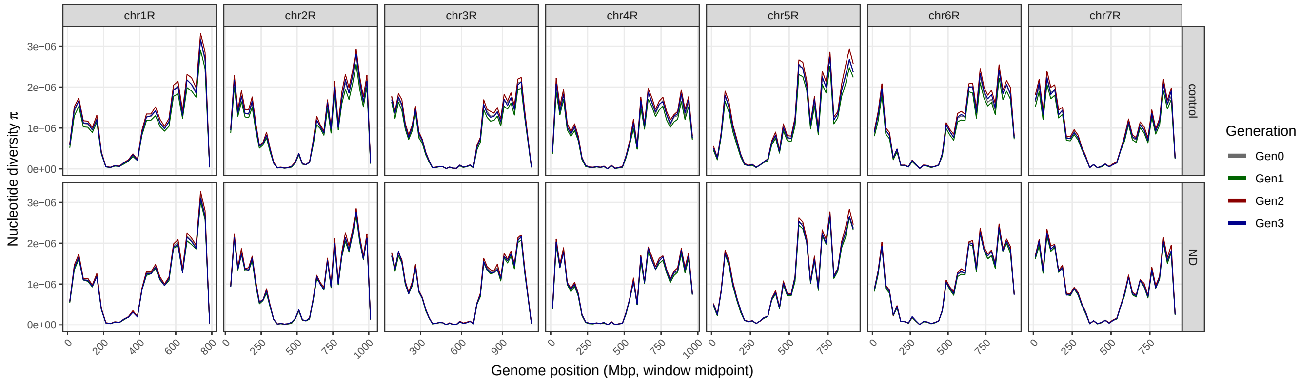
Nucleotide diversity per 25 Mbp window
