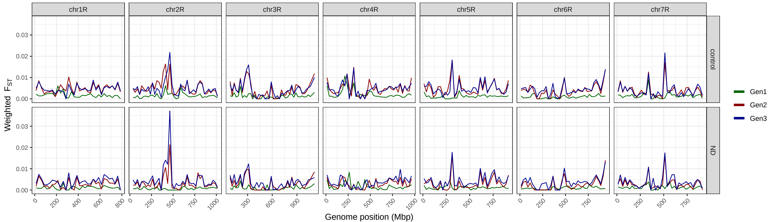
F_{ST} versus Gen0
