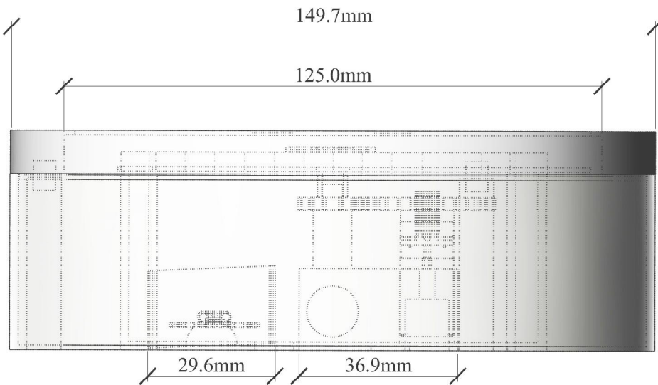
Top View 1:1.25
