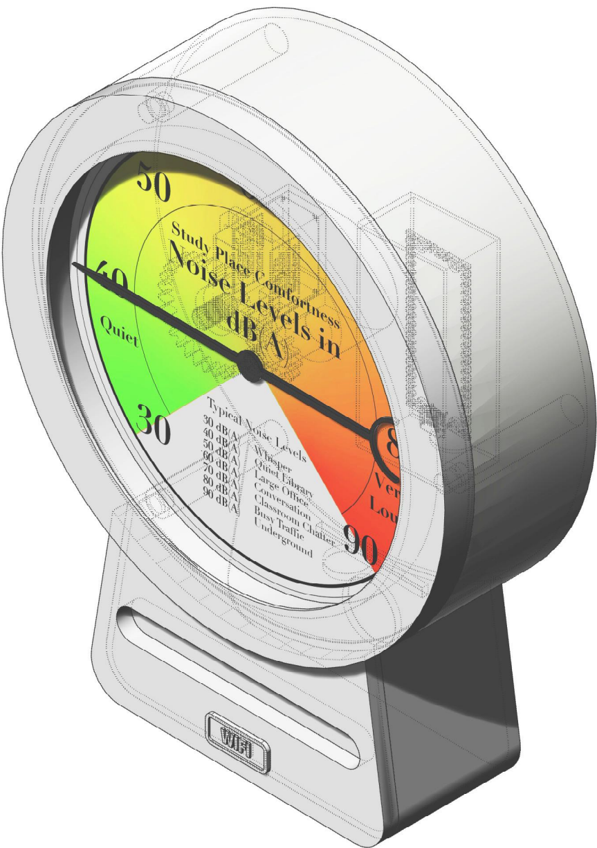
Isometric View 1:1.25
