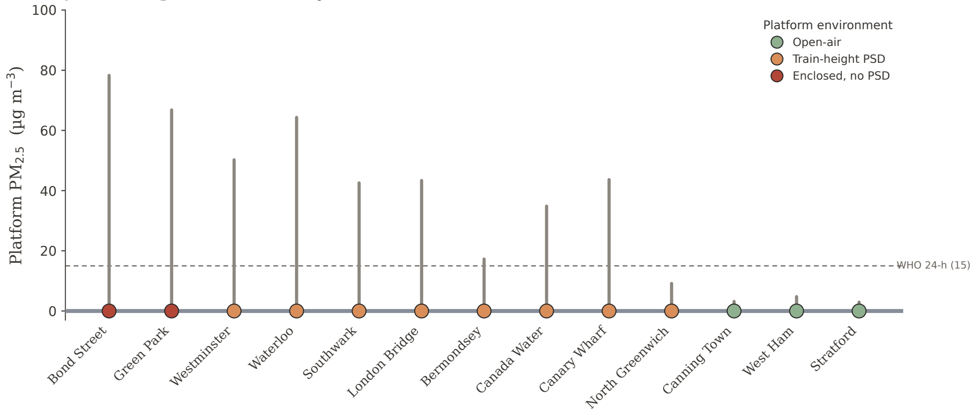
Jubilee — platform PM 2.5 by station (route order)
