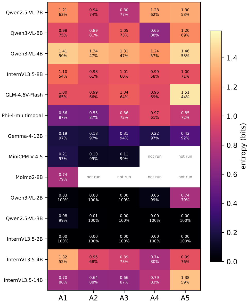
Output entropy and majority share (GT-independent)
