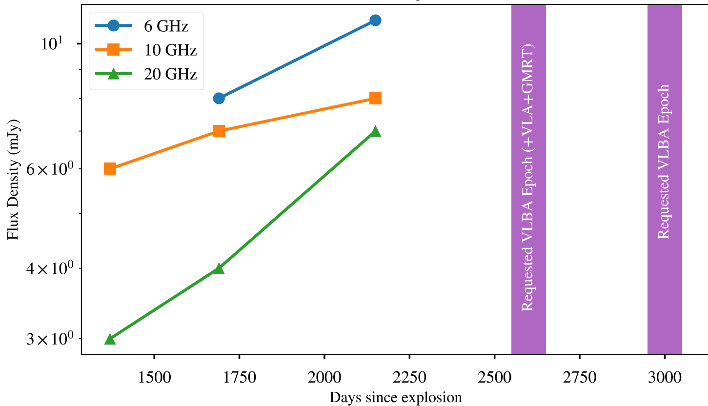
SN 2018ivc Lightcurves
