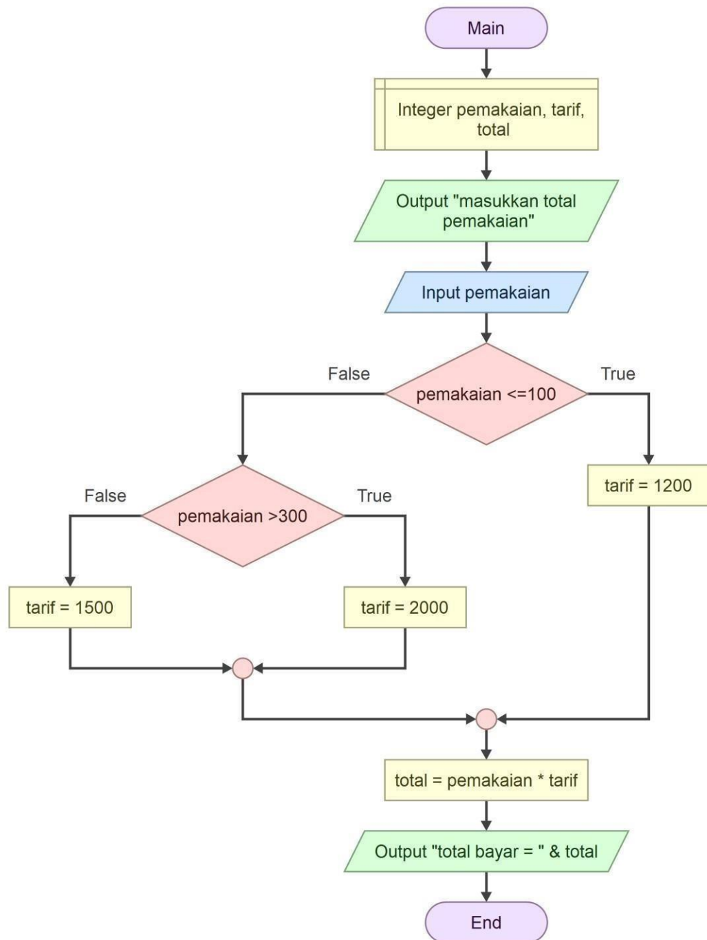
Gambar 1.1 Flowchart
