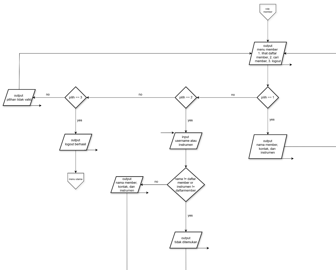
Gambar 1.5 Flowchart pada menu member
