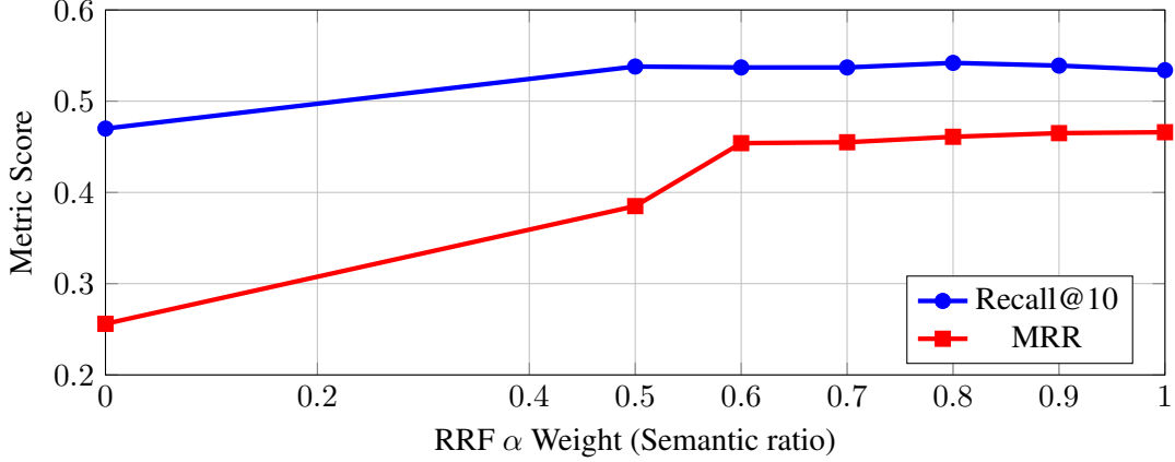
Figure 5: Effect of RRF \alpha parameter on Retrieval Quality. \alpha = 0 represents pure keyword, while \alpha = 1 is pure semantic search. Setting \alpha = 0.80 offers the highest top-10 boundary.
