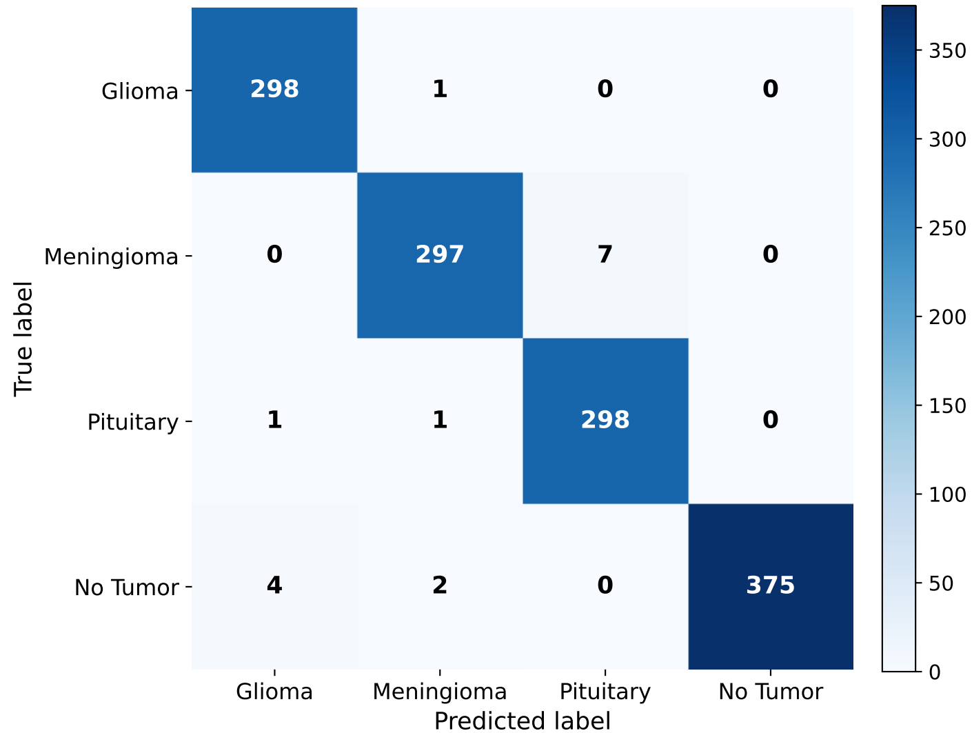
Confusion Matrix
