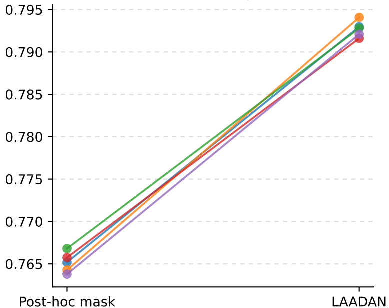
Paired return by seed
