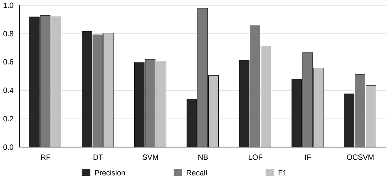
Precision, Recall and F1 on the main process holdout
